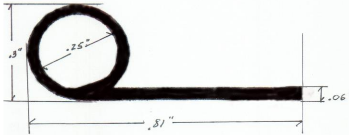
GT131 Extruded Silicone "P" Seal 5/16" x 13/16" ±0.039"
